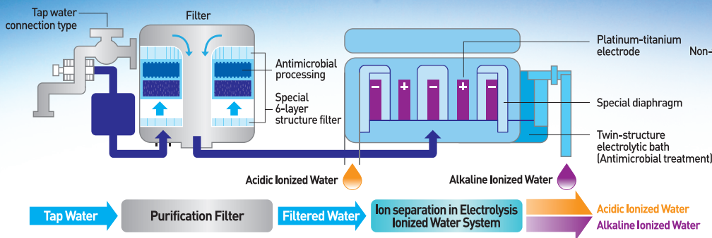
[ Diagram of the Mechanism for Ionized Water Production ]
